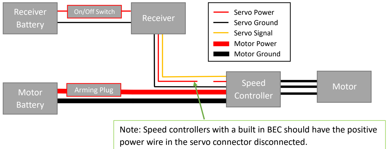
Figure 2.3: Example diagram of propulsion system with Arming Plug. Note, different classes may have additional requirements or allow for alternative configurations.
